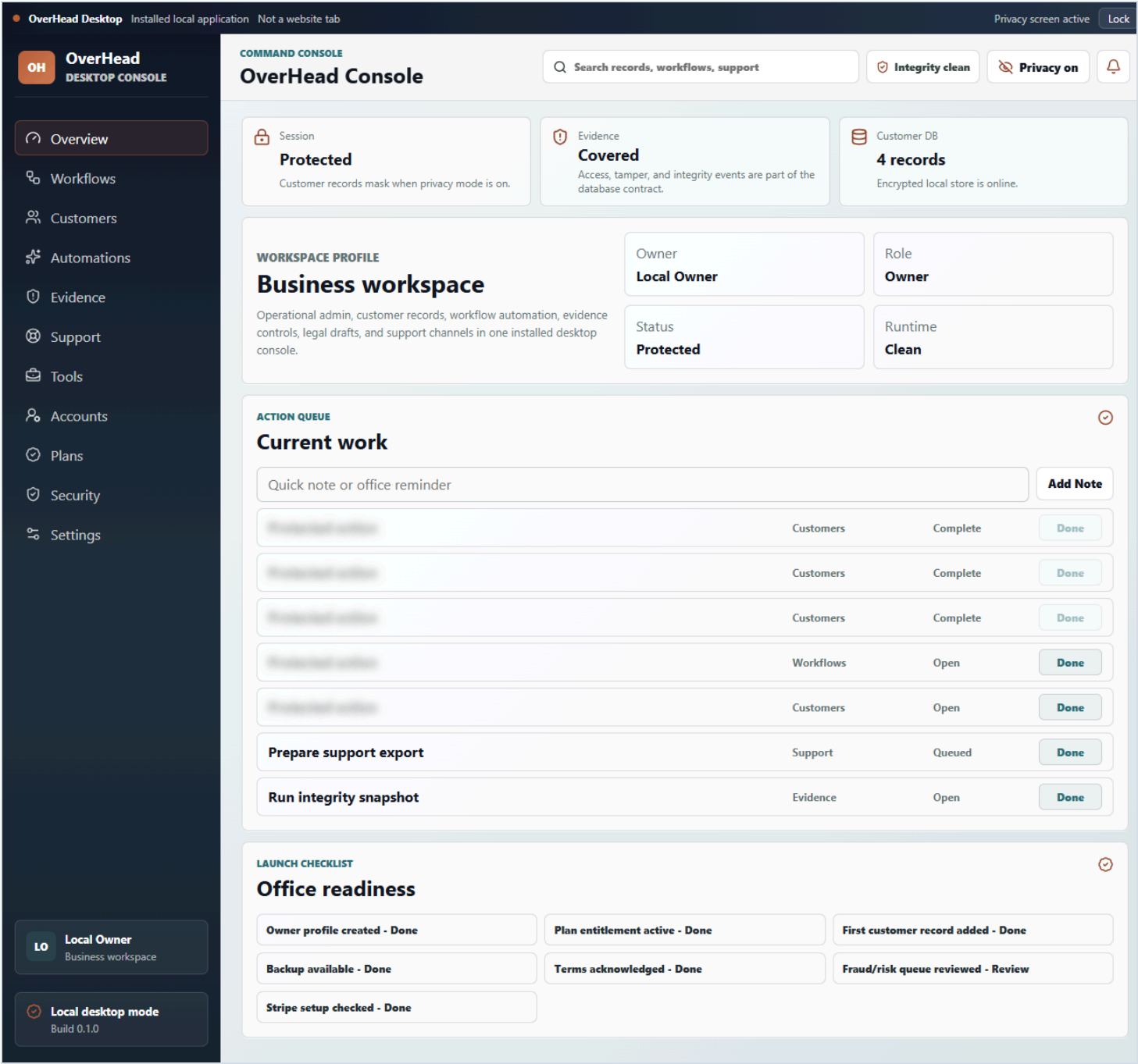
OverHead Desktop smoke-test capture: signed-in command console with workspace status, customer database, current work, office readiness, and security indicators.
