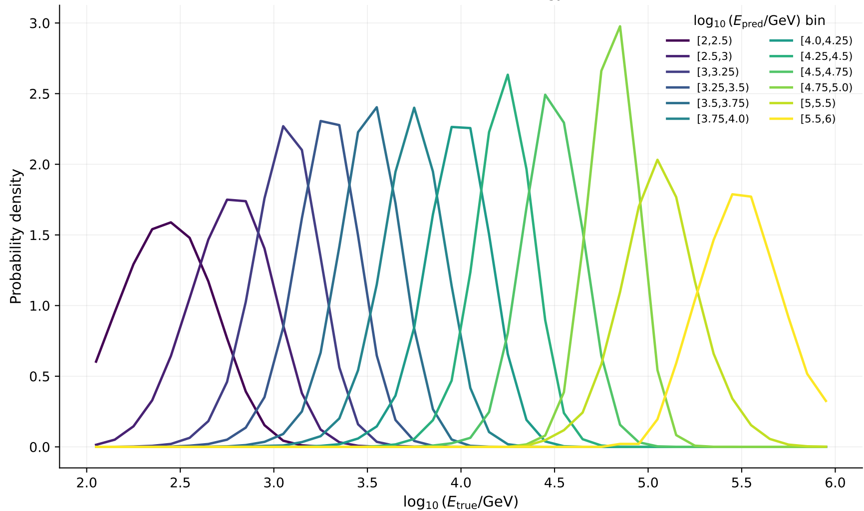
v6 selected cells: normalized true-energy distributions
