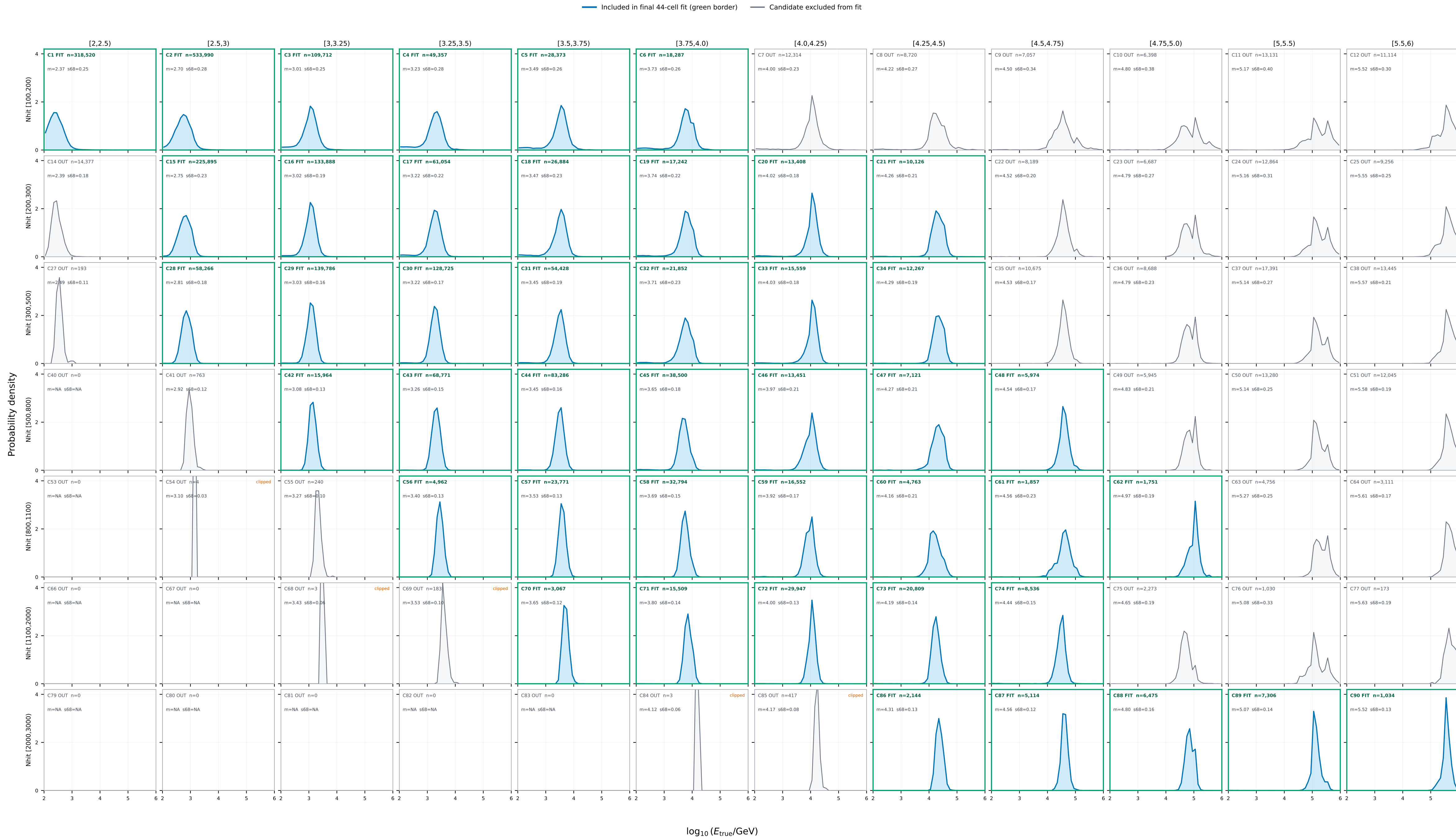
v6 64748: normalized true-energy distributions for 84 candidate cells
