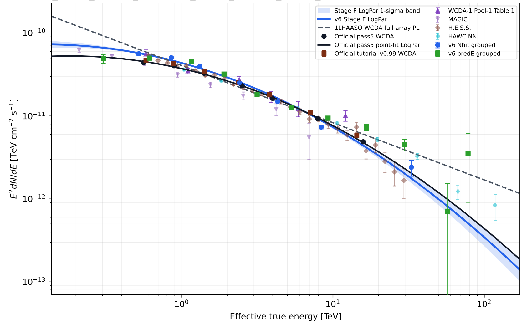
Stage G v6_64748_nhit100_reselect44_split56_miss030_double_rayleigh SED overlay: Nhit + predE group
