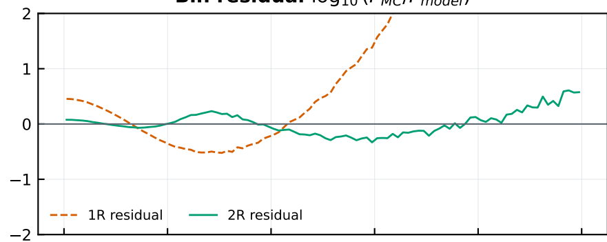
Bin residual \log_{10}(P_{MC}/P_{model})
