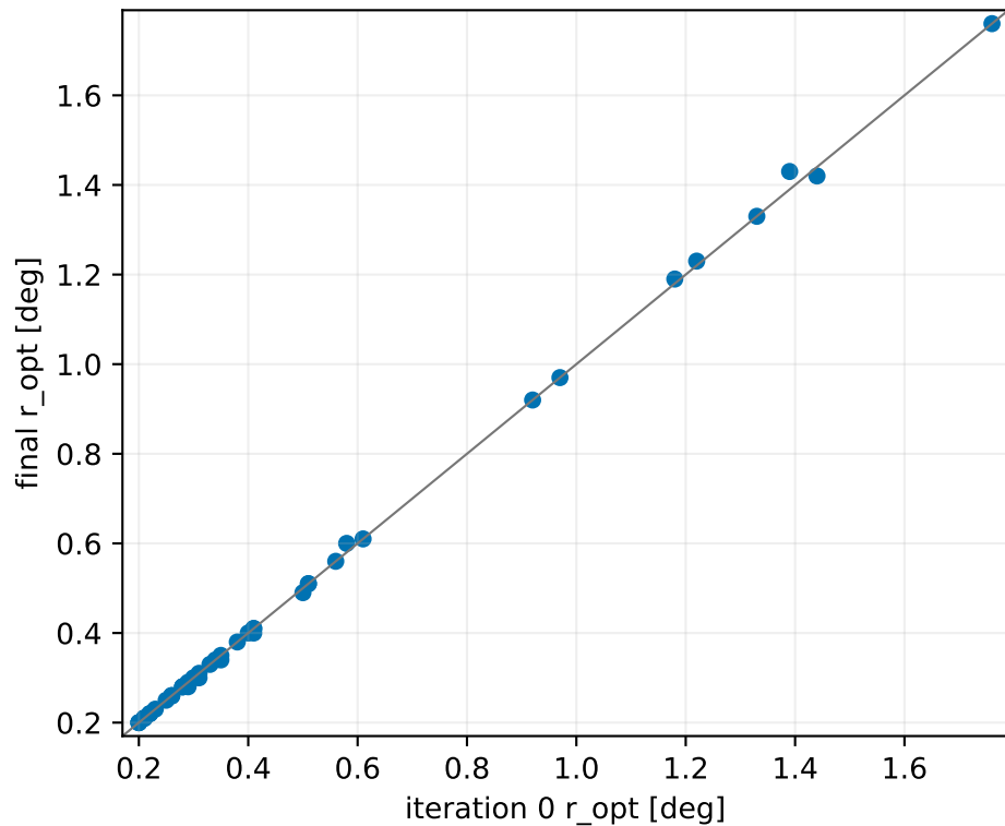
Aperture-radius stability
