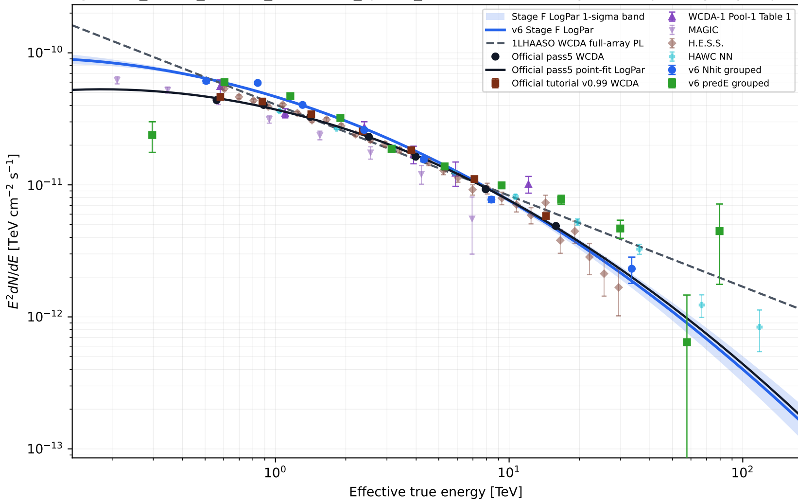
Stage G v6_64748_nh100_reselect44_split56_miss030 SED overlay: Nh1t + predE grouped points
