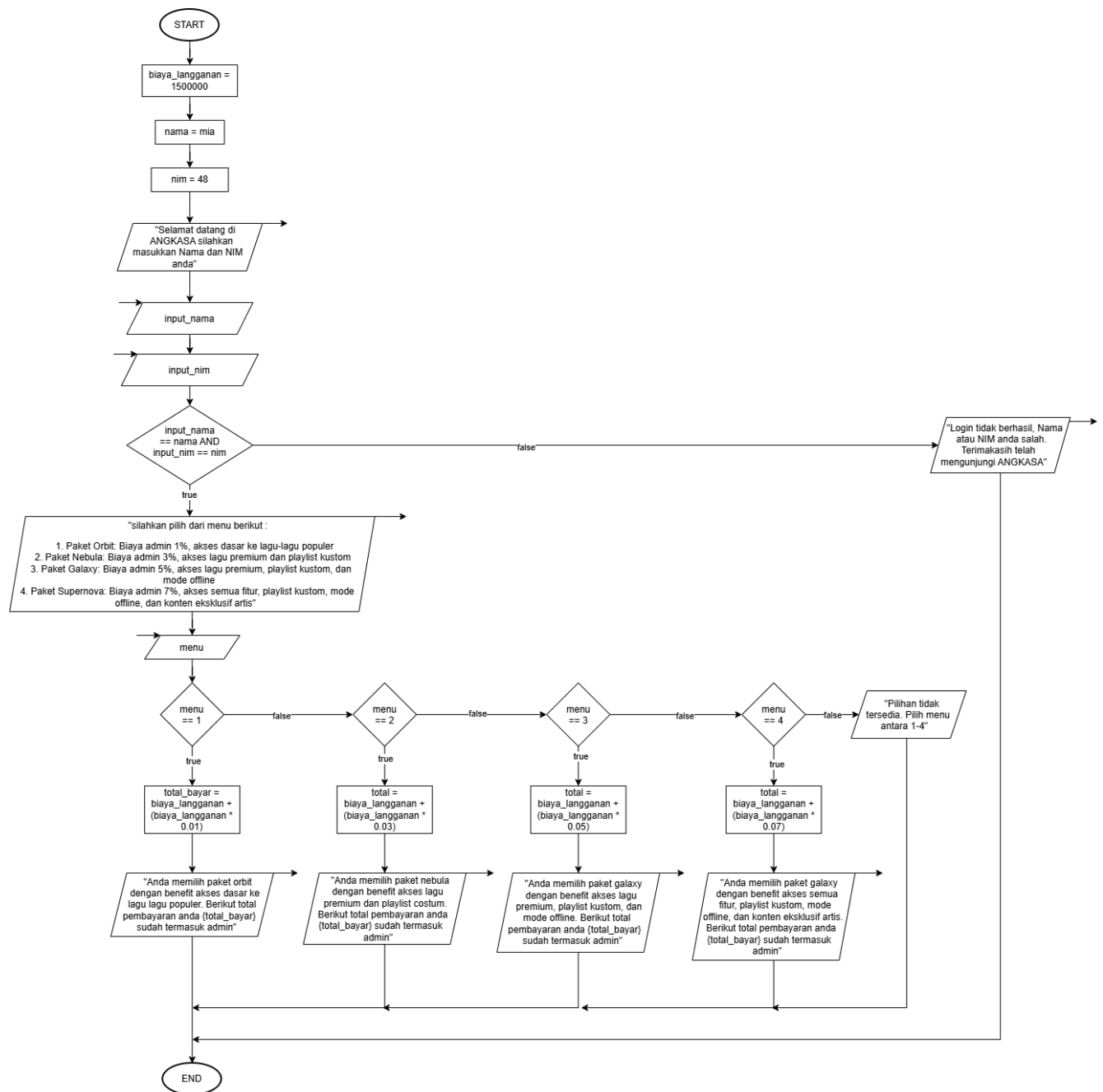
Gambar 1.1 Flowchart
