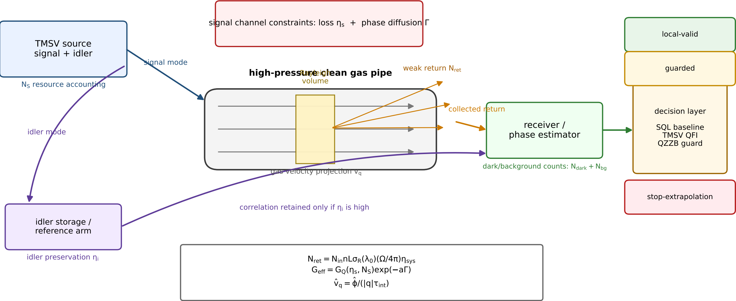
The schematic separates the macro photon budget, microscopic quantum-channel boundary, detector admissibility, and global QZZB guardrail.
