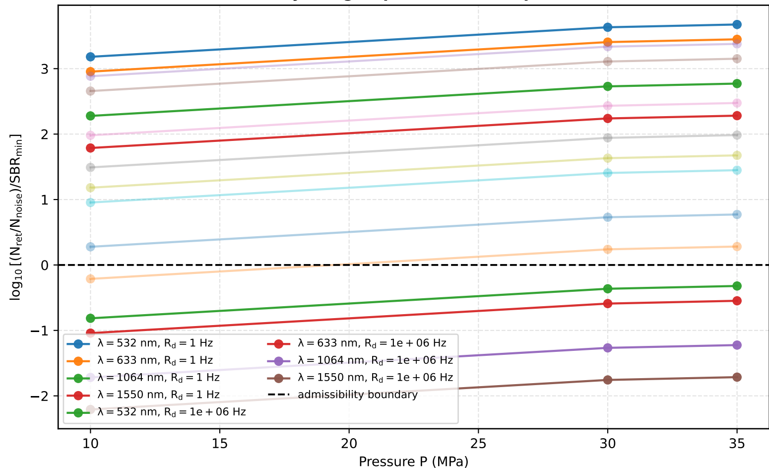
Detector admissibility margin: positive values pass the SBR criterion
