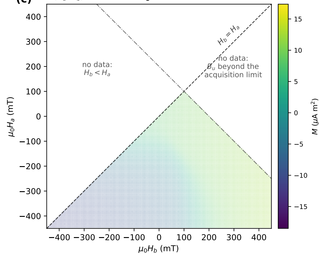
(c) M(H_a, H_b) measurement grid
