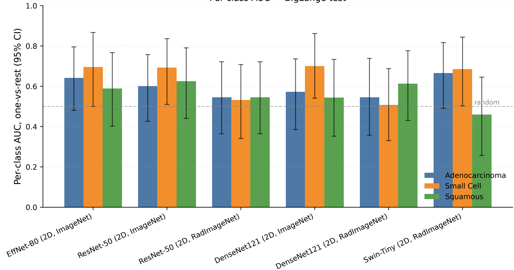
Per-class AUC — BigLunge test
