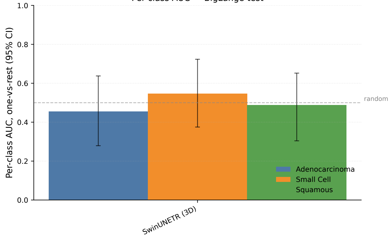
Per-class AUC — BigLunge test
