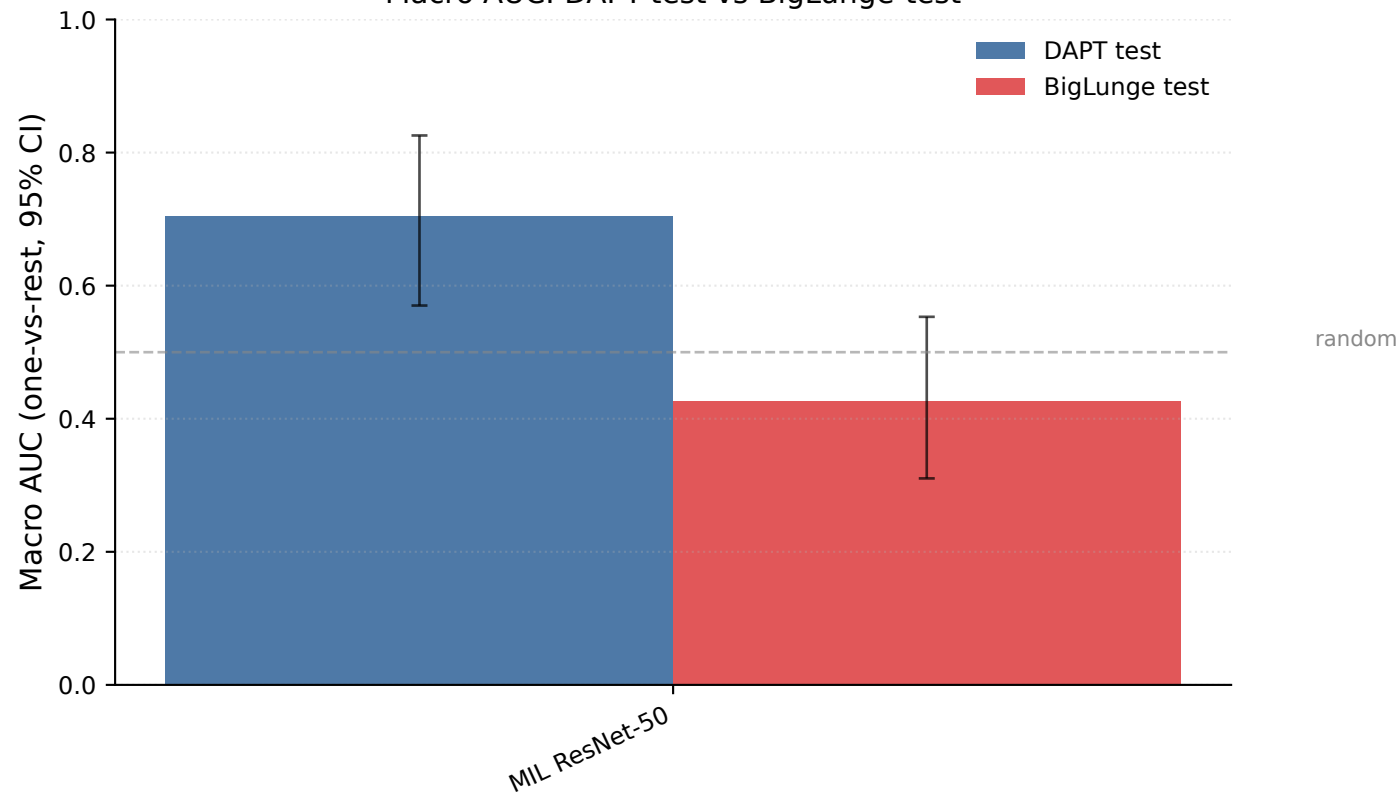
Macro AUC: DAPT-test vs BigLunge-test
