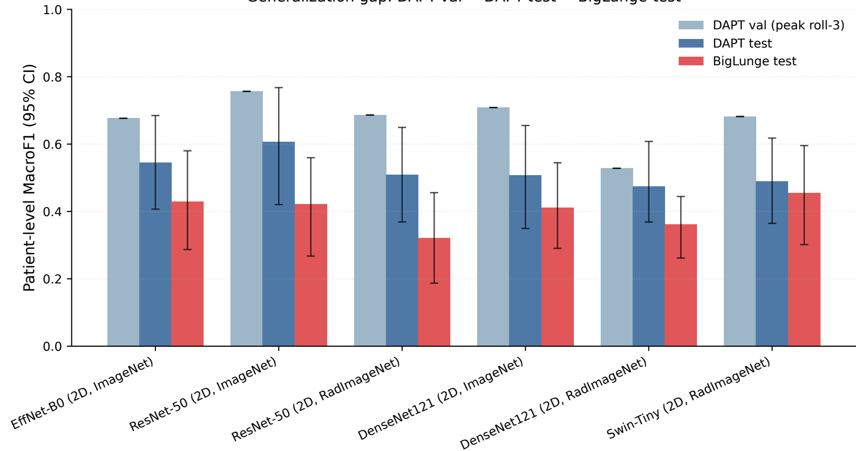
Generalization gap: DAPT-val \rightarrow DAPT-test \rightarrow BigLunge-test
