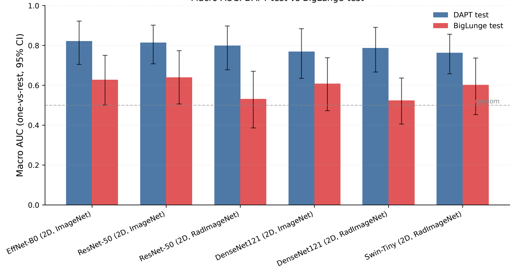
Macro AUC: DAPT-test vs BigLunge-test
