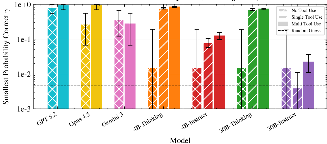
LLM Performance ( p = 12, d = 4, g = 31 )
