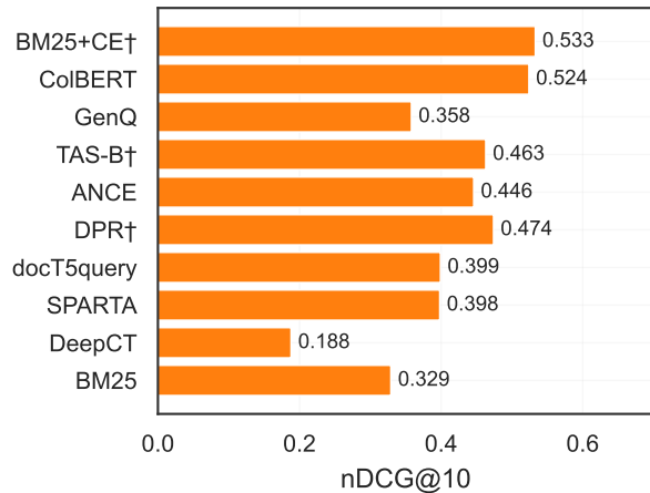
BEIR Benchmark (Table 2)
