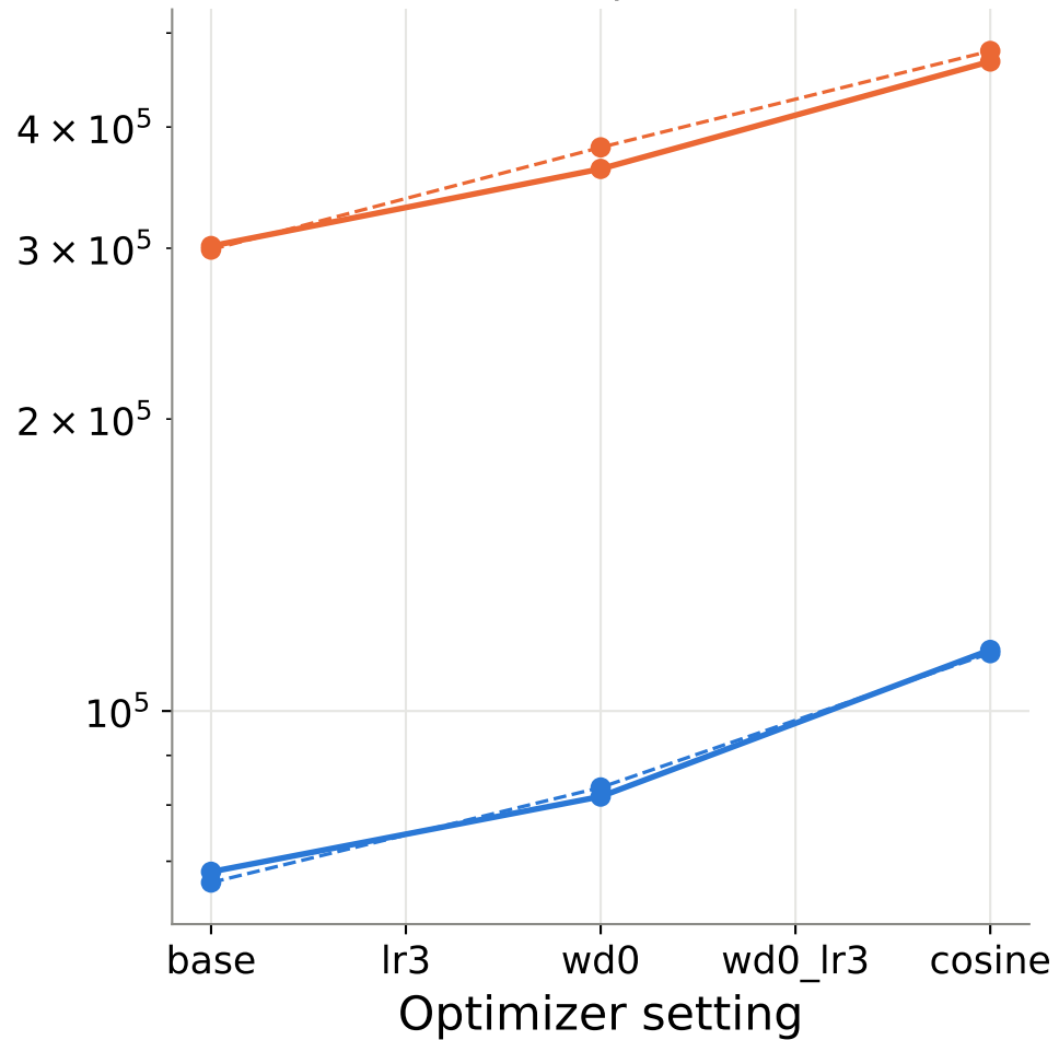
L (31.5M params)
