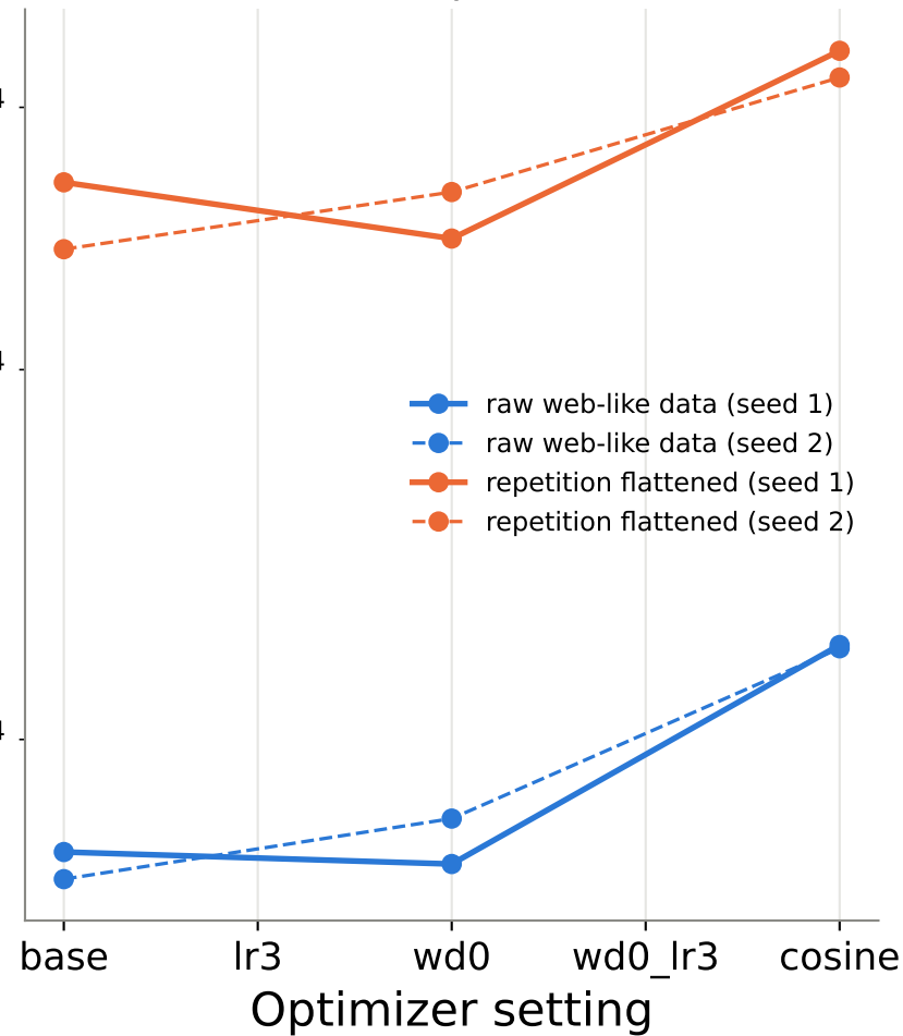
S (2.0M params)
