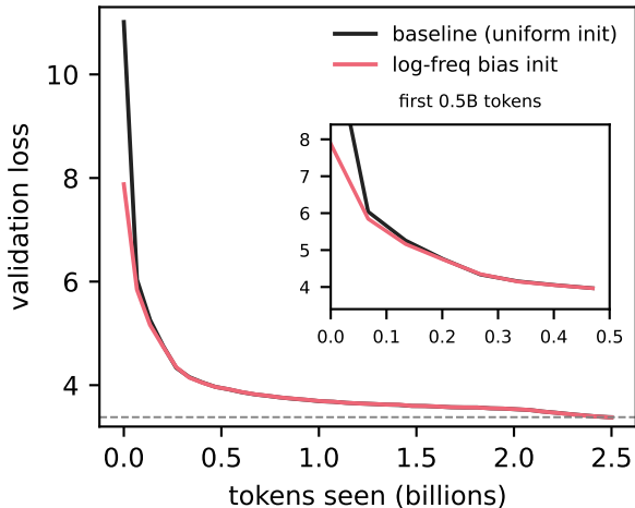
Log-frequency bias init (A40)
