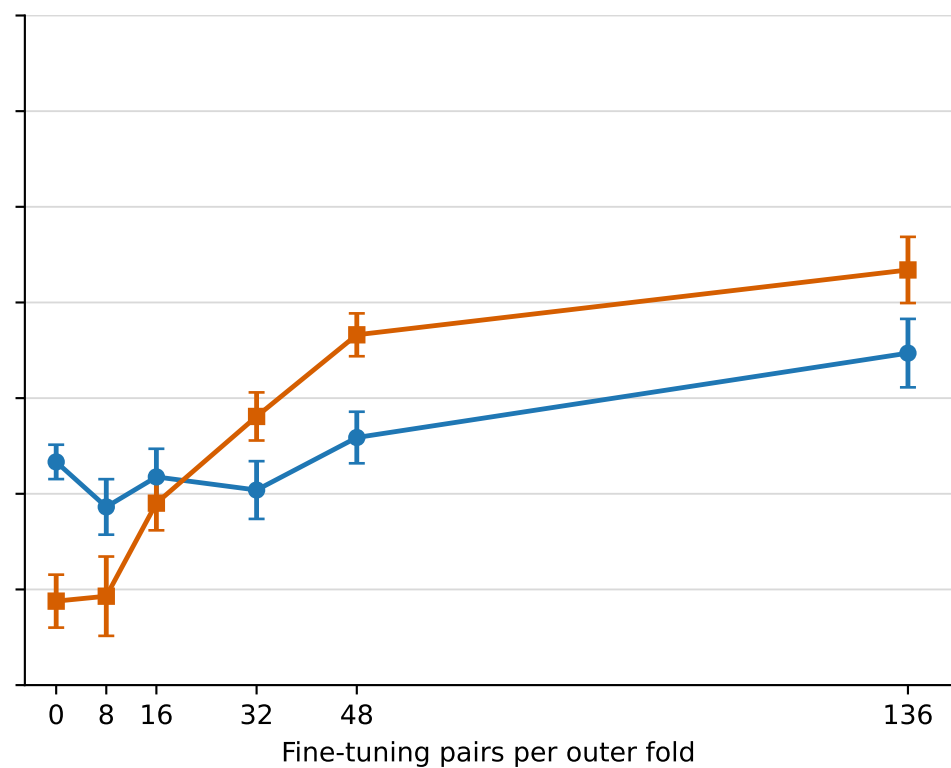
Four-class classification
