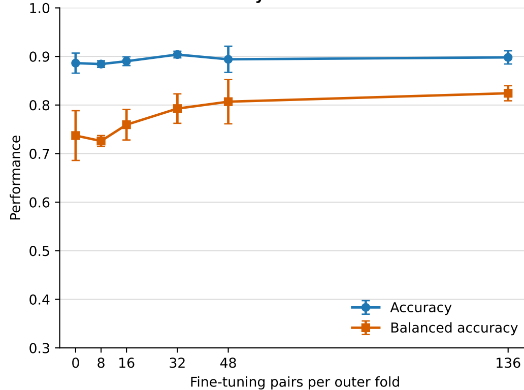
Binary classification
