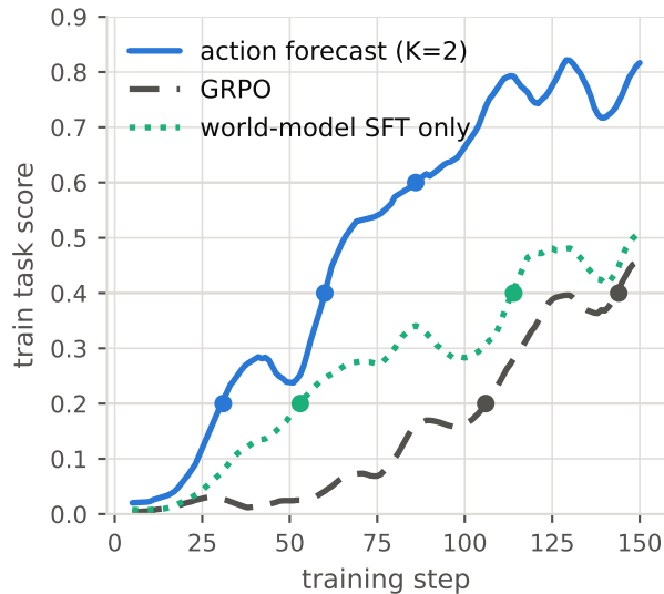
sample efficiency
