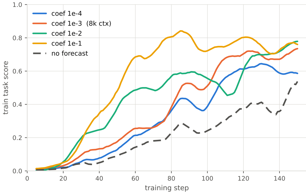
SciWorld, K=3: action-forecast loss coefficient
