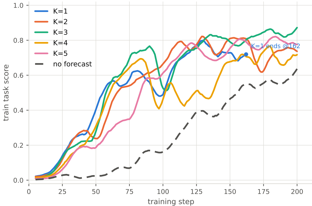
SciWorld: forecast horizon K (smoothed over 10 steps)
