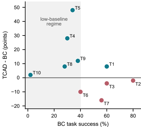
Task-level gain is largest where BC is weak
