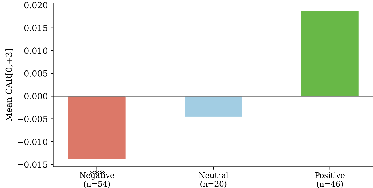
Mean Abnormal Returns by LLM Sentiment Group (NGX, 2020-2024; *** p < 0.01 , ** p < 0.05 , * p < 0.10 ) ***
