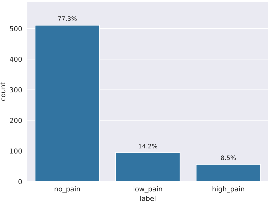
Label Distribution
