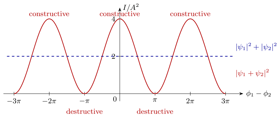
Figure 2: The interference term. The resulting intensity depends on the relative phase \phi_1 - \phi_2 : constructive interference produces maxima, while destructive interference produces minima.
