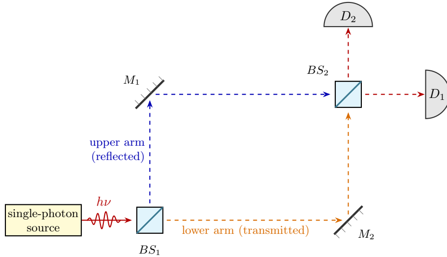
Figure 14: Mach-Zehnder interferometer. BS_1 and BS_2 are 50/50 beam splitters; M_1 and M_2 are fully reflecting mirrors. The colored lines show the two available routes, not two pieces of a photon; the red dashed lines mark the two output ports leading to the detectors D_1 and D_2 .
