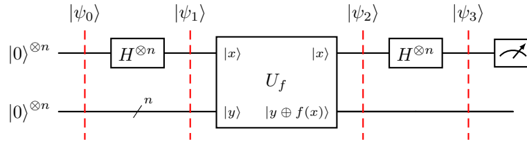
Figure 21: Quantum circuit for Simon's algorithm.
