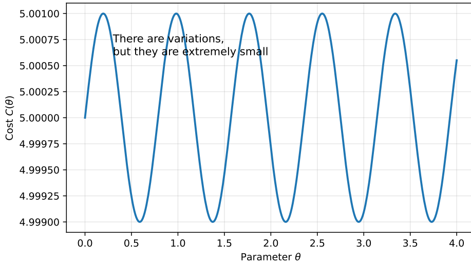
Figure 30: A barren plateau is not perfectly flat. There are small hills and valleys, but they are so small that the optimizer cannot distinguish them from numerical noise.
