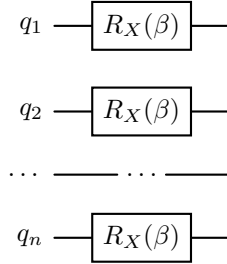
Figure 35: Circuit implementing the Mixer Layer U_M(\beta) for n qubits.
