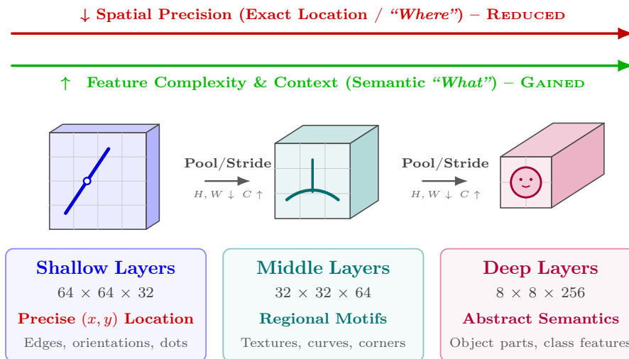
Figure 87: Evolution of CNN representations with depth. As the network becomes deeper, spatial resolution H \times W decreases while the number of feature maps C typically increases. Larger receptive fields and progressive downsampling shift the representation from spatially precise, low-level features toward increasingly contextual and higher-level patterns, reducing the importance of exact feature location.
