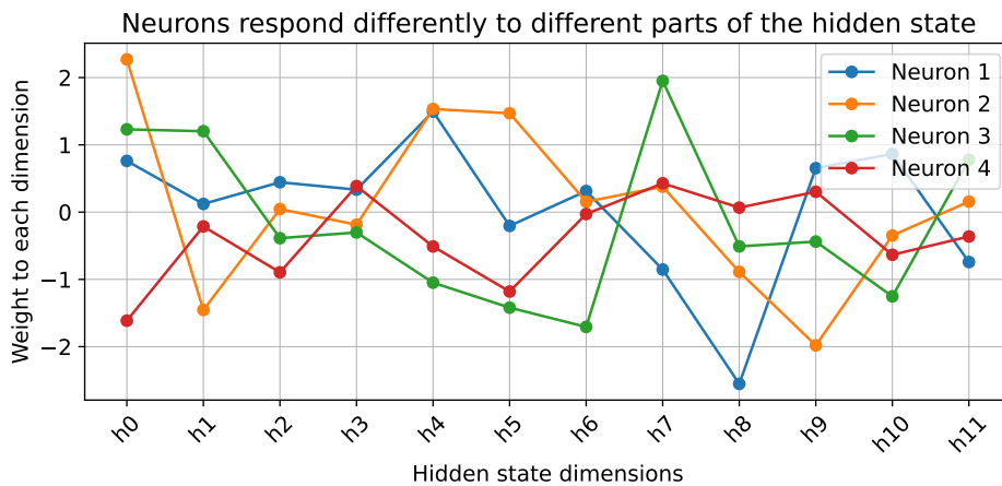
Figure 30: Line plot of 4 different neurons (lines), each extracting different information from the same hidden state vector (x-axis). The y-values represent the weight magnitudes, showing how each neuron focuses on different parts of the hidden state to extract unique features. So even though all neurons receive the same hidden state vector h , they do different things with it , they extract different aspects of the stored memory.
