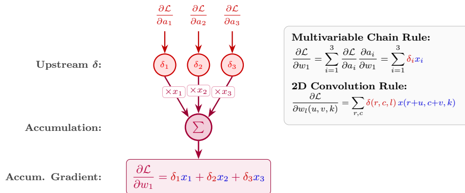
Figure 88: Weight sharing and gradient accumulation in convolutional layers. A single kernel parameter is reused across multiple spatial locations during the forward pass; consequently, during backpropagation, its gradient accumulates the contributions from all output activations that depend on that shared parameter.
