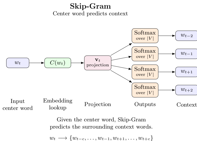
Figure 43: Skip-Gram architecture in Word2Vec. [11]
