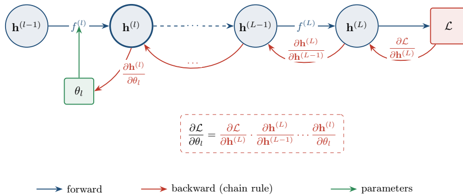
Figure 88: Backpropagation through a CNN. The forward pass computes activations from layer l to the loss, while the backward pass applies the chain rule in reverse to obtain \frac{\partial \mathcal{L}}{\partial \theta_l} , multiplying the local derivatives of all subsequent layers.
