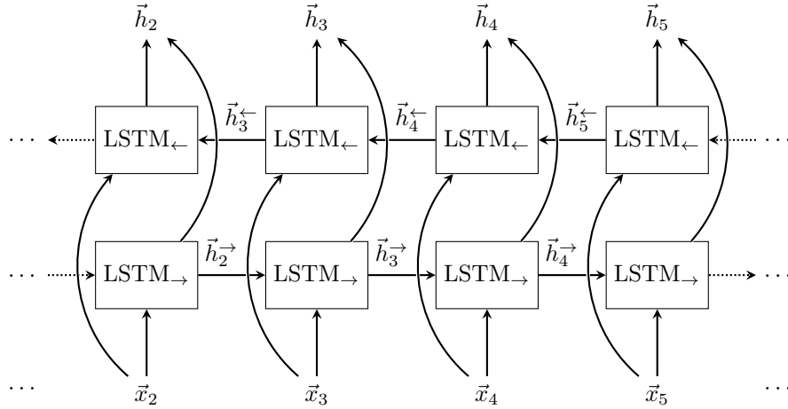
Figure 37: Bidirectional LSTM (BiLSTM) architecture. [10] The input sequence \{x_t\} is processed by two independent LSTM chains operating in opposite directions.
