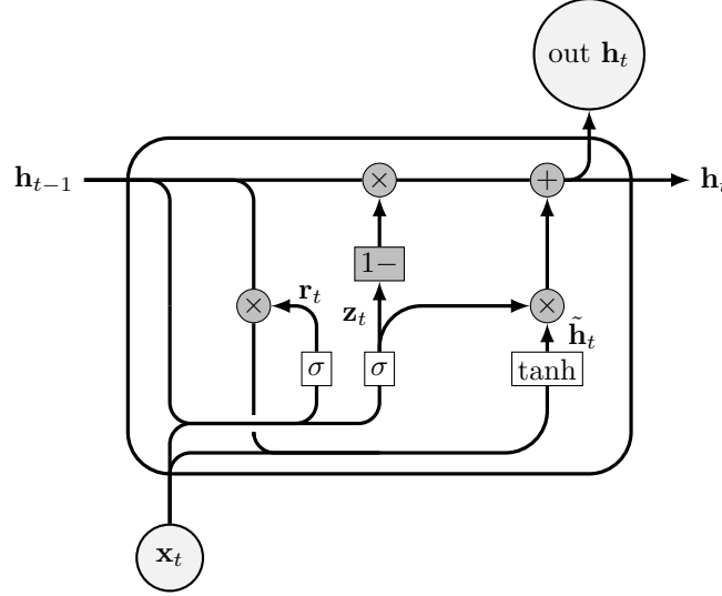
Figure 34: Gated Recurrent Unit (GRU) cell. [8] At time step t , the GRU receives the current input x_t and the previous hidden state h_{t-1} , and computes the new hidden state h_t , which serves both as output and as recurrent input to the next time step.
