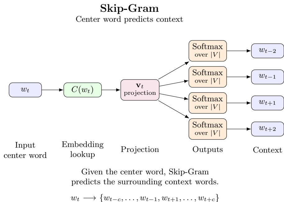
Figure 43: Skip-Gram architecture in Word2Vec. [11]
