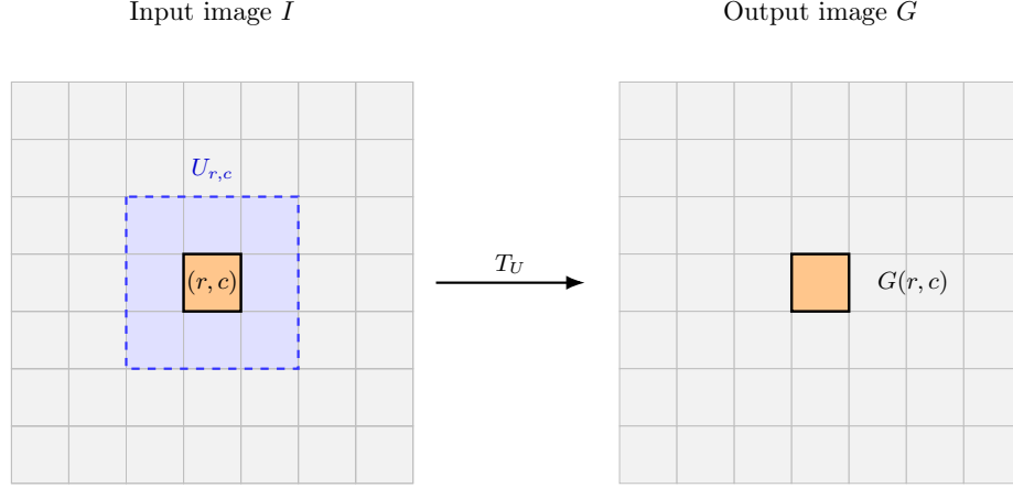
Figure 47: A local transformation T_U that computes the output pixel G(r, c) from the input image I using only the local neighbourhood U_{r,c} .
