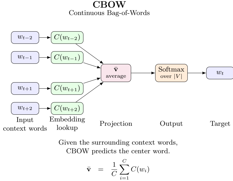
Figure 42: CBOW architecture in Word2Vec. [12]
