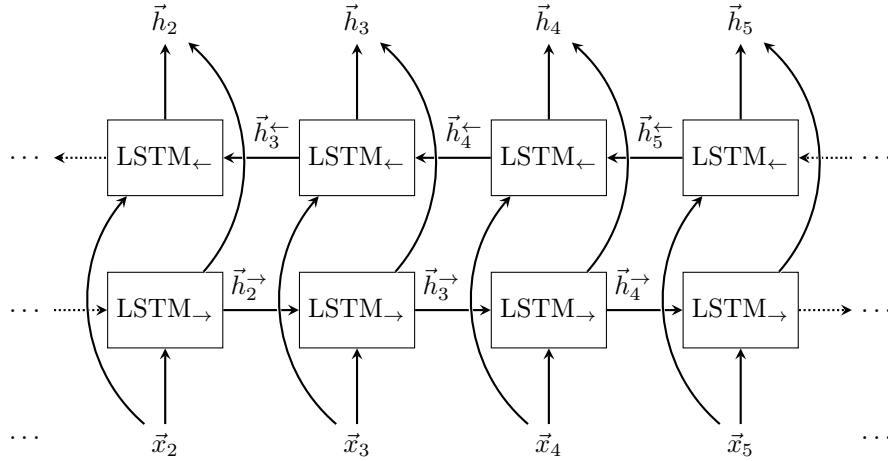
Figure 37: Bidirectional LSTM (BiLSTM) architecture. [14] The input sequence \{x_t\} is processed by two independent LSTM chains operating in opposite directions.
