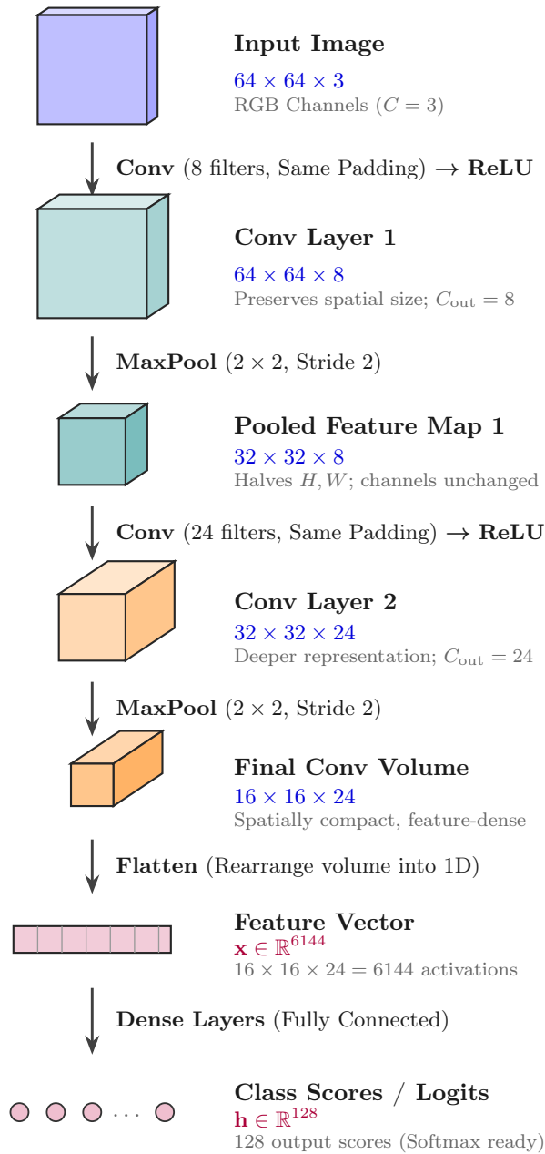
Figure 73: Step-by-step shape transformation across a Convolutional Neural Network. The spatial dimensions ( H, W ) shrink via Max Pooling while channel depth ( C ) increases through learned convolutions, culminating in a 1D flattened feature vector for dense classification.
