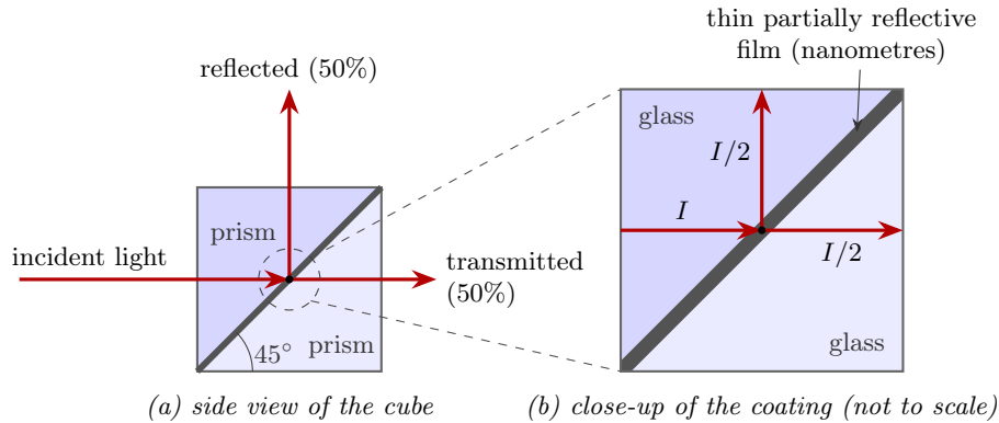
Figure 12: How a beam splitter works. (a) A beam-splitter cube is made of two glass prisms joined along their diagonal. The light hits the interface at 45^\circ : half of the intensity is transmitted straight on, and half is reflected at 90^\circ . (b) Close-up of the interface: the “partially reflective mirror” is a very thin coating, only a few nanometres thick, which reflects part of the light and lets the rest through. For a 50/50 beam splitter, the coating is tuned so that an incident intensity I leaves as I/2 + I/2 .
