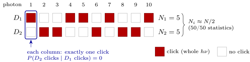
Figure 13: Anticorrelated detector clicks at a 50/50 beam splitter. (a) A single photon of energy h\nu is detected whole, at D_1 or at D_2 , never at both and never split: P(D_1 \text{ and } D_2) = 0 . Dashed lines mark the two possible output ports, not a trajectory the photon is known to follow. (b) An illustrative sequence of detections. Read by columns, the record shows anticorrelation (one click per photon); read by rows, it shows the 50/50 statistics N_1 \approx N_2 \approx N/2 (real runs fluctuate around N/2 ).
