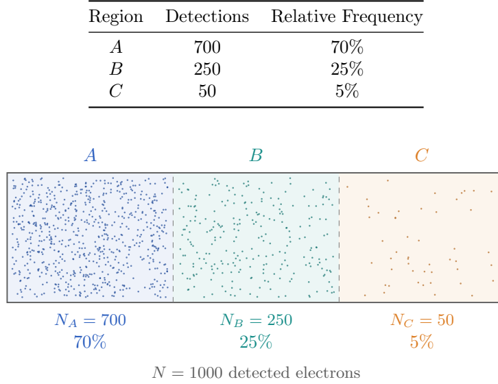
Figure 7: Relative frequencies of electron detections. A fluorescent screen is divided into three equal-sized regions A , B , and C . After N = 1000 detections, the hypothetical counts are N_A = 700 , N_B = 250 , and N_C = 50 , corresponding to relative frequencies of 70%, 25%, and 5%. Each dot represents one localized electron detection. All values are illustrative.
