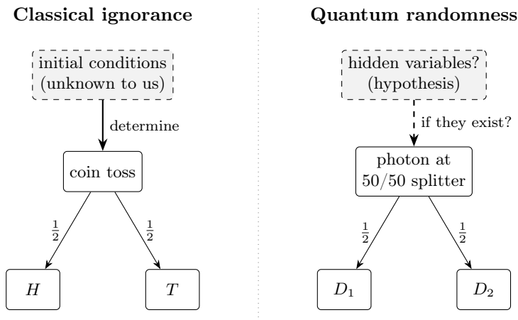
Figure 10: Both situations give a 50/50 distribution, but only in the classical case do we know the randomness comes from missing information.
