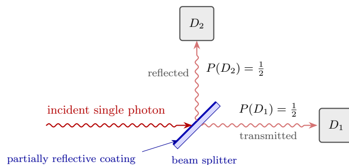
Figure 11: A single photon at a 50/50 beam splitter. The two outputs are equally likely detection outcomes, and each photon is detected at exactly one detector.
