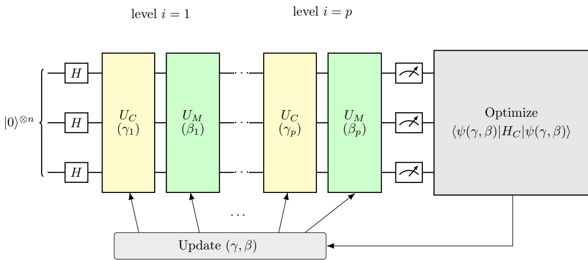
Figure 29: Structure of the QAOA ansatz.
