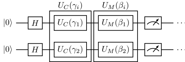
Figure 30: QAOA ansatz with one layer ( p = 1 ) for two qubits ( n = 2 ).
