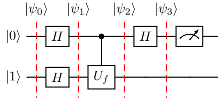
Figure 17: Deutsch's Algorithm. The final measurement of the data qubit reveals whether the function is constant or balanced.
