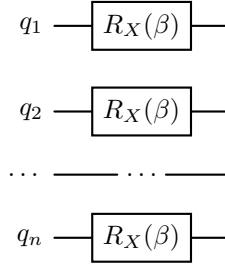
Figure 33: Circuit implementing the Mixer Layer U_M(\beta) for n qubits.
