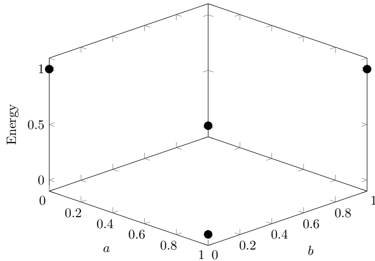
Figure 19: Discrete energy landscape of the QUBO formulation for the boolean function a \neq b . The ground states correspond to the minimum-energy configurations (0, 1) and (1, 0) .
