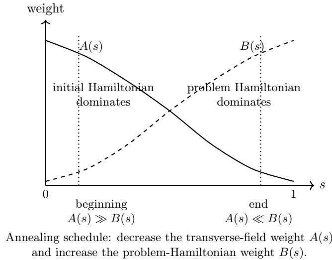
Figure 22: Typical annealing schedule controlled by the functions A(s) and B(s) .
