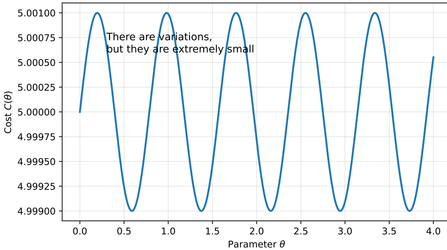
Figure 28: A barren plateau is not perfectly flat. There are small hills and valleys, but they are so small that the optimizer cannot distinguish them from numerical noise.
