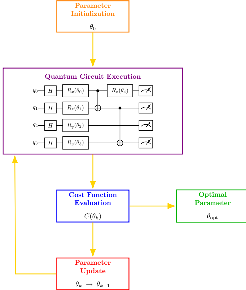
Figure 24: Schematic representation of the iterative optimization loop in a Variational Quantum Algorithm. The process starts with parameter initialization, followed by quantum circuit execution, cost function evaluation, and parameter update. The loop continues until convergence to the optimal parameters \theta_{\text{opt}} .
