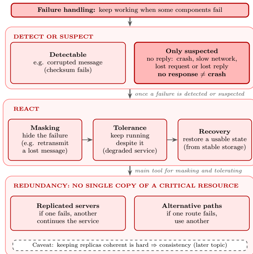
Figure 6: Failure handling: detect or suspect, react, and redundancy.
