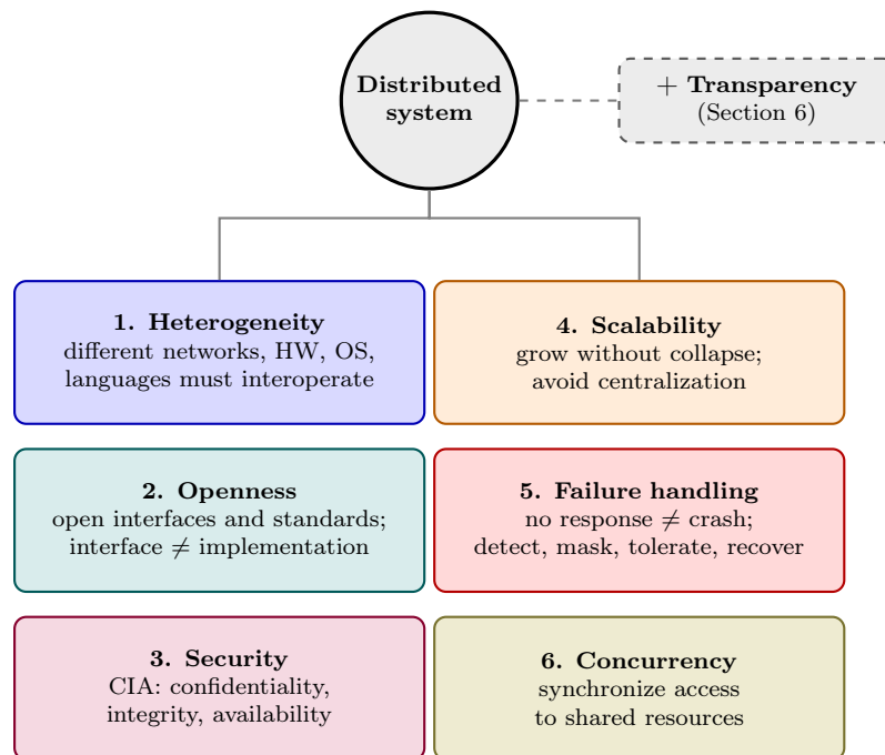
Figure 3: Main challenges of distributed systems.
