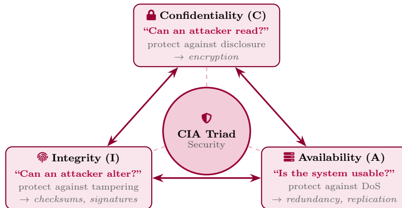
Figure 4: The CIA triad: core security objectives in distributed systems.
