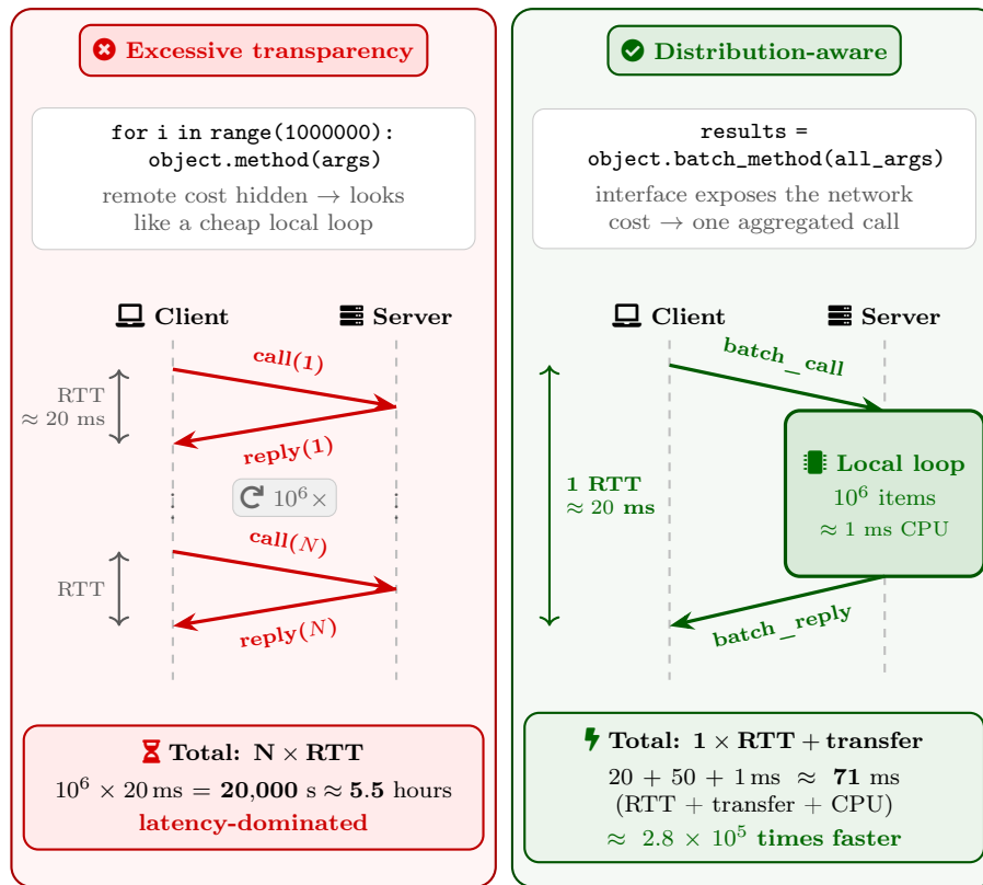
Figure 9: The latency trap (illustrative numbers). Excessive transparency can hide network latency and encourage inefficient fine-grained remote calls; exposing distribution costs enables batching and better performance.
