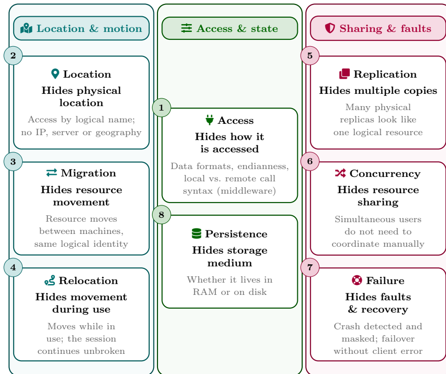
Figure 8: Taxonomy of transparency : the eight forms grouped by the aspect of distribution they hide.
