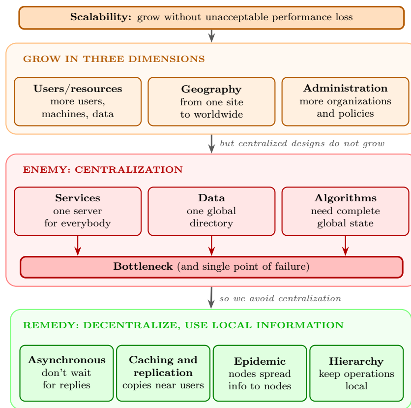
Figure 5: Scalability: dimensions, enemy and remedies.
