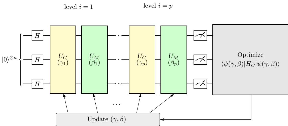
Figure 28: Structure of the QAOA ansatz.
