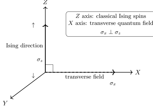
Figure 22: The quantum field acts along the X direction, perpendicular to the Ising Z direction.
