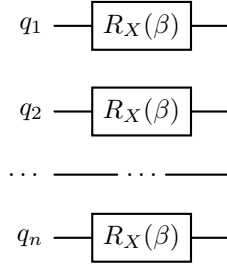
Figure 34: Circuit implementing the Mixer Layer U_M(\beta) for n qubits.
