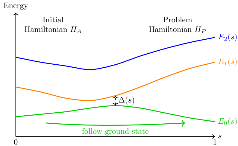
Figure 24: Schematic representation of the evolution of the eigenspectrum during Quantum Annealing. The curves represent the energy levels E_0(s) , E_1(s) , and E_2(s) as functions of the annealing parameter s . The gap \Delta(s) between the ground state and the first excited state is called the Spectral Gap , and it measures how far the ground state is from the first excited state . Gap is important because the smaller the gap becomes ( \Delta \approx 0 ), the easier it is for the system to jump from the ground state to an excited state, which can lead to errors in the computation.
