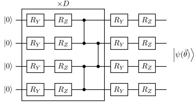
Figure 26: Generic Hardware Efficient Ansatz on 4 qubits. The final R_Y and R_Z gates are an additional final rotation layer. They are placed after the repeated entangling block because, after entanglement has been created, we may still want to independently adjust each qubit before measuring or evaluating the cost function.
