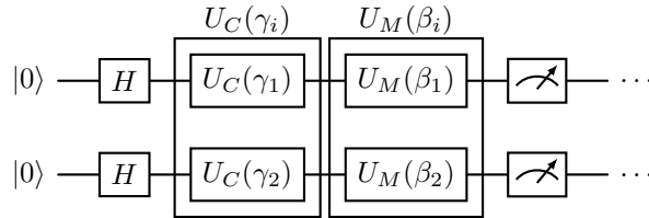
Figure 31: QAOA ansatz with one layer ( p = 1 ) for two qubits ( n = 2 ).
