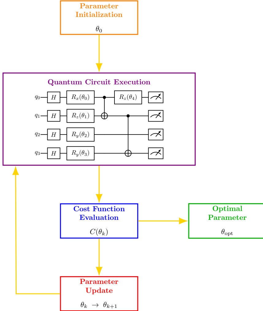
Figure 25: Schematic representation of the iterative optimization loop in a Variational Quantum Algorithm. The process starts with parameter initialization, followed by quantum circuit execution, cost function evaluation, and parameter update. The loop continues until convergence to the optimal parameters \theta_{\text{opt}} .
