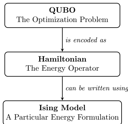
Figure 21: Relationship between QUBO, Hamiltonian, and Ising model.
