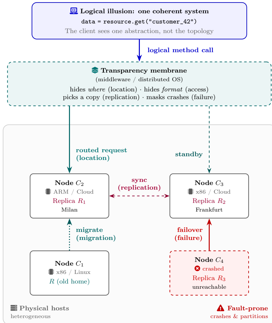
Figure 7: Distributed-system transparency: a logical resource is presented as a single coherent abstraction while middleware hides selected details of its physical distribution, such as location, representation, migration, replication, and failures.
