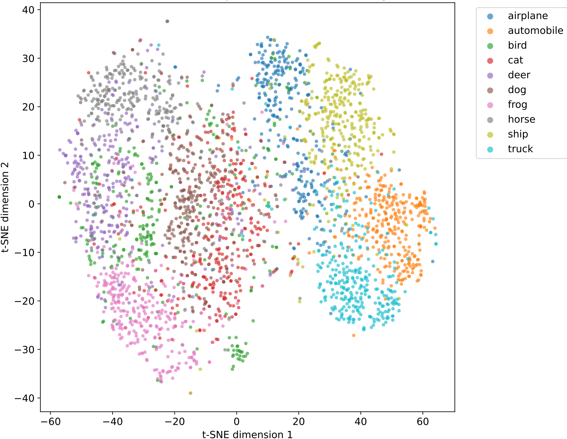
CIFAR-10 t-SNE from pretrained CNN embeddings
