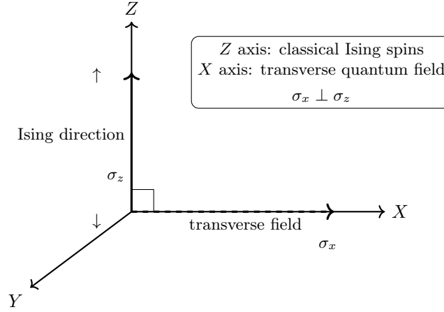
Figure 24: The quantum field acts along the X direction, perpendicular to the Ising Z direction.
