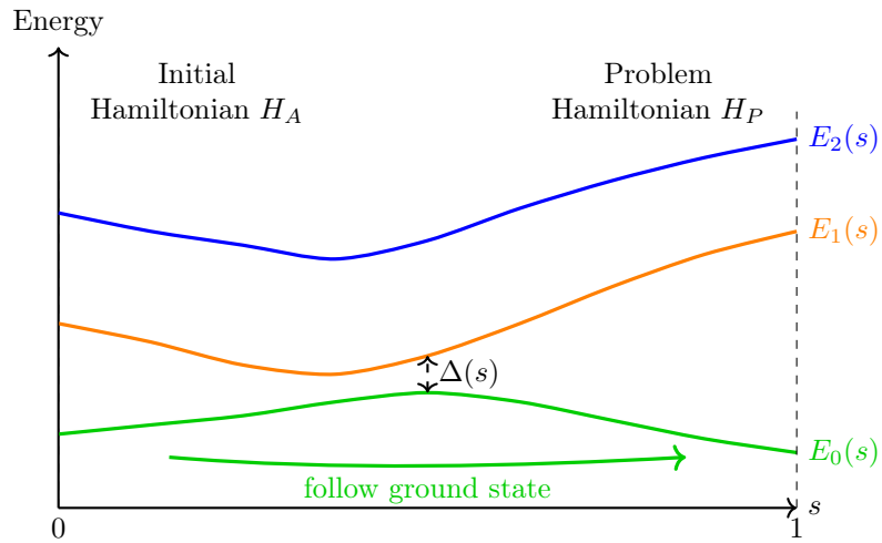
Figure 26: Schematic representation of the evolution of the eigenspectrum during Quantum Annealing. The curves represent the energy levels E_0(s) , E_1(s) , and E_2(s) as functions of the annealing parameter s . The gap \Delta(s) between the ground state and the first excited state is called the Spectral Gap , and it measures how far the ground state is from the first excited state . Gap is important because the smaller the gap becomes ( \Delta \approx 0 ), the easier it is for the system to jump from the ground state to an excited state, which can lead to errors in the computation.
