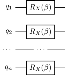
Figure 36: Circuit implementing the Mixer Layer U_M(\beta) for n qubits.
