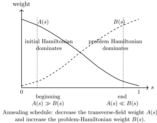
Figure 25: Typical annealing schedule controlled by the functions A(s) and B(s) .
