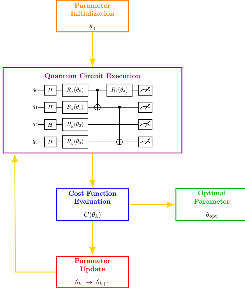
Figure 27: Schematic representation of the iterative optimization loop in a Variational Quantum Algorithm. The process starts with parameter initialization, followed by quantum circuit execution, cost function evaluation, and parameter update. The loop continues until convergence to the optimal parameters \theta_{\text{opt}} .
