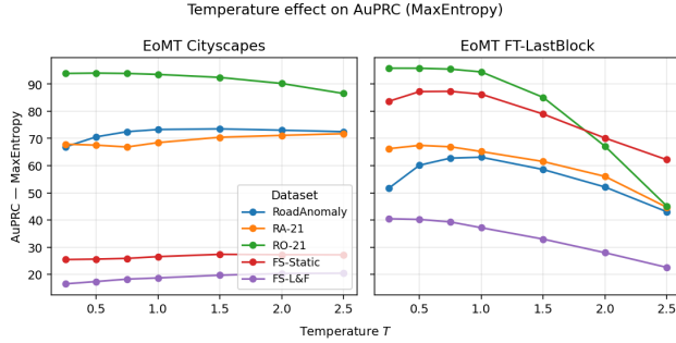
Figure 2. MaxEntropy AuPRC under temperature scaling.
