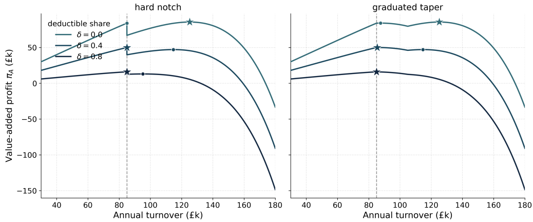
Figure 8: Optima of the value-added (formulation A) profit function (4), \pi_A(y) = (1 - \delta)(1 - \tau f(y))y - C(y; n, e) , at statutory rate \tau = 0.20 , ability n = £130k and elasticity e = 0.17 , under the hard registration notch (left) and the graduated taper (right). Each panel overlays three deductible-input shares \delta \in \{0.0, 0.4, 0.8\} ; dots mark each curve's local maxima and the star its global optimum, and the dashed vertical line is the £85,000 threshold. The value-added factor (1 - \delta) scales the whole curve down without moving the frictionless optimum, while a higher \delta shrinks the retained wedge (1 - \delta)(1 - \tau) and so pulls the registered optimum y^* = n[(1 - \delta)(1 - \tau)]^e back toward the threshold—eventually tipping the global optimum from the registered interior peak to bunching at the notch, consistent with the formulation-A discussion above.
