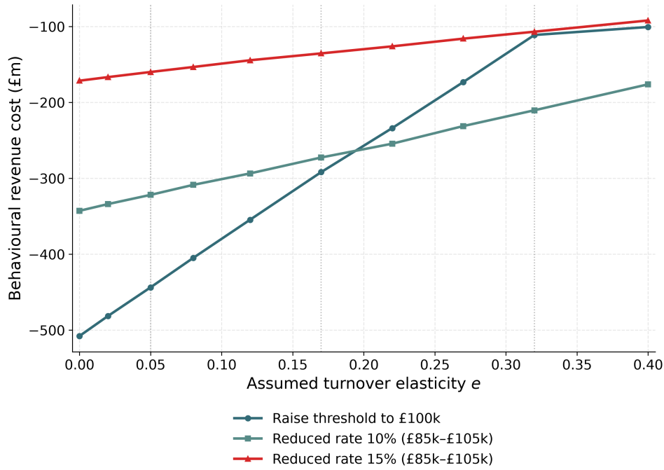
Figure 9: Behavioural reform cost against the assumed turnover elasticity e , for the three flat-rate reforms. Each curve is the change in revenue relative to the £85,000-notch baseline as e varies; the intercept at e = 0 is the static cost of Table 2, onto which the behavioural cost nests as the response vanishes. As e rises, firms scale turnover up toward their frictionless optimum (6), broadening the taxed base and making each reform cheaper. The dotted lines mark the swept values e \in \{0.05, 0.17, 0.32\} of Table 3. The graduated taper is omitted: its behavioural response is not credibly identified in this framework (see above). All magnitudes are conditional on the assumed, non-identified e .
