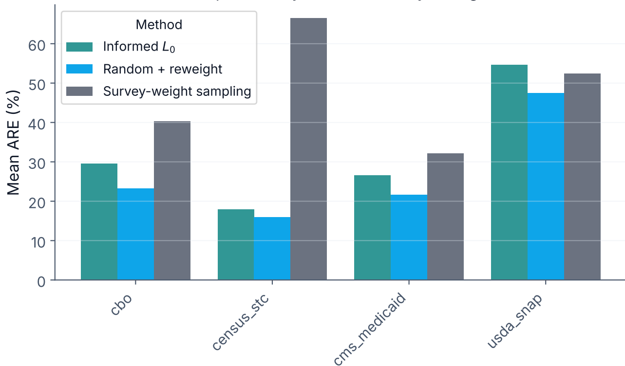
Out-of-sample ARE by held-out family (budget 10,000)
